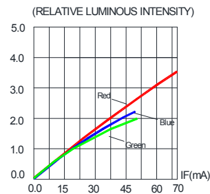
FIG.2 RELATIVE LUMINOUS INTENSITY VS. FORWARD CURRENT
