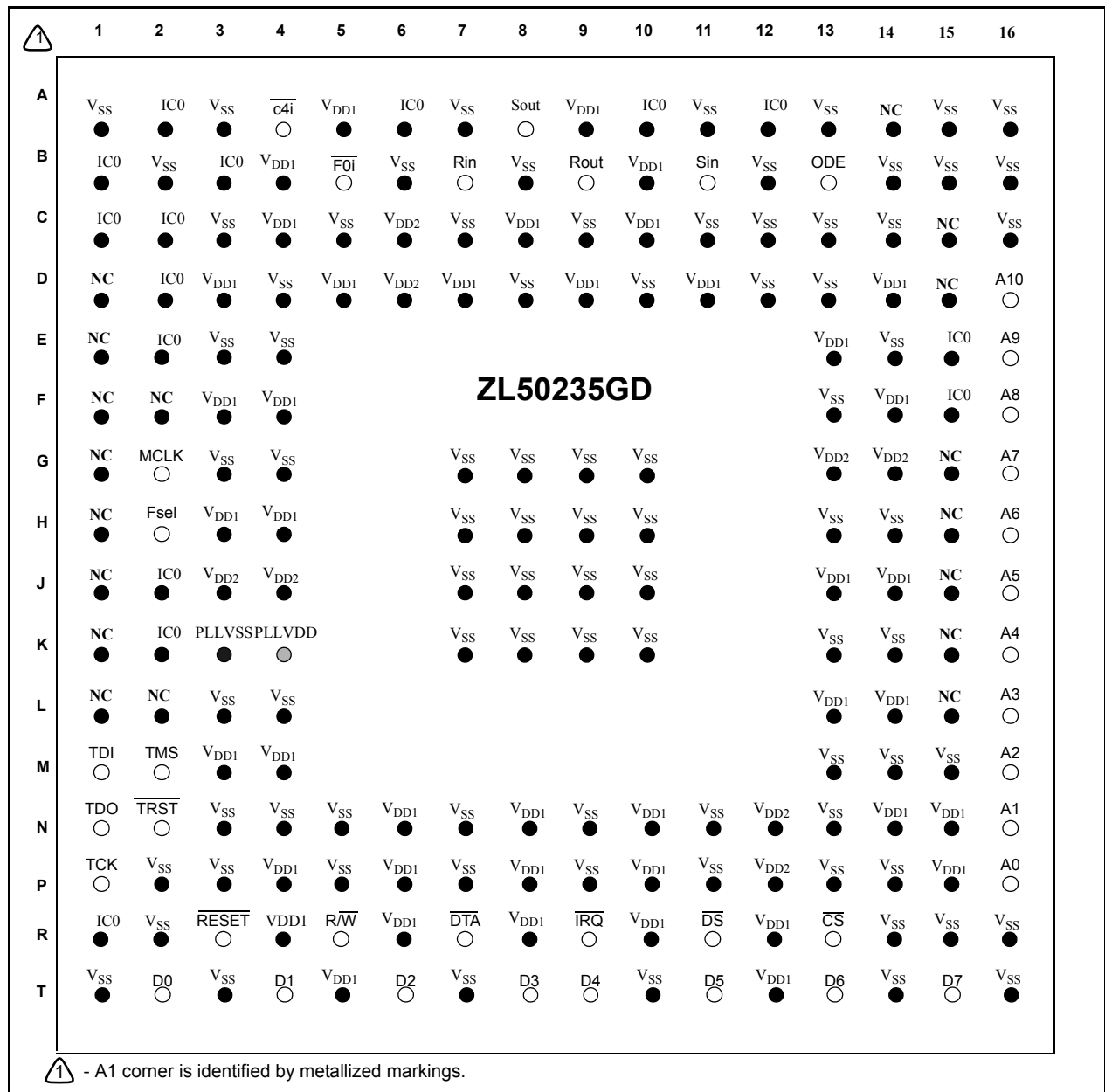
Figure 3 - 208 Ball LBGA
