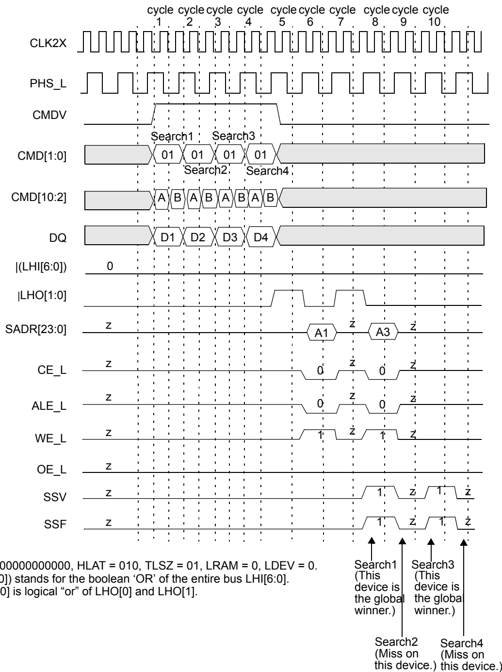
Figure 10-6. Timing Diagram for 72-bit Search Device Number 0
