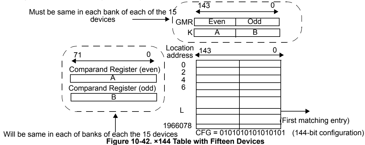
Figure 10-42. \times 144 Table with Fifteen Devices
