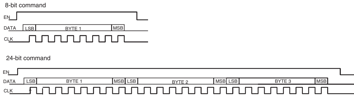
Figure 3-8. Pulse Diagram
