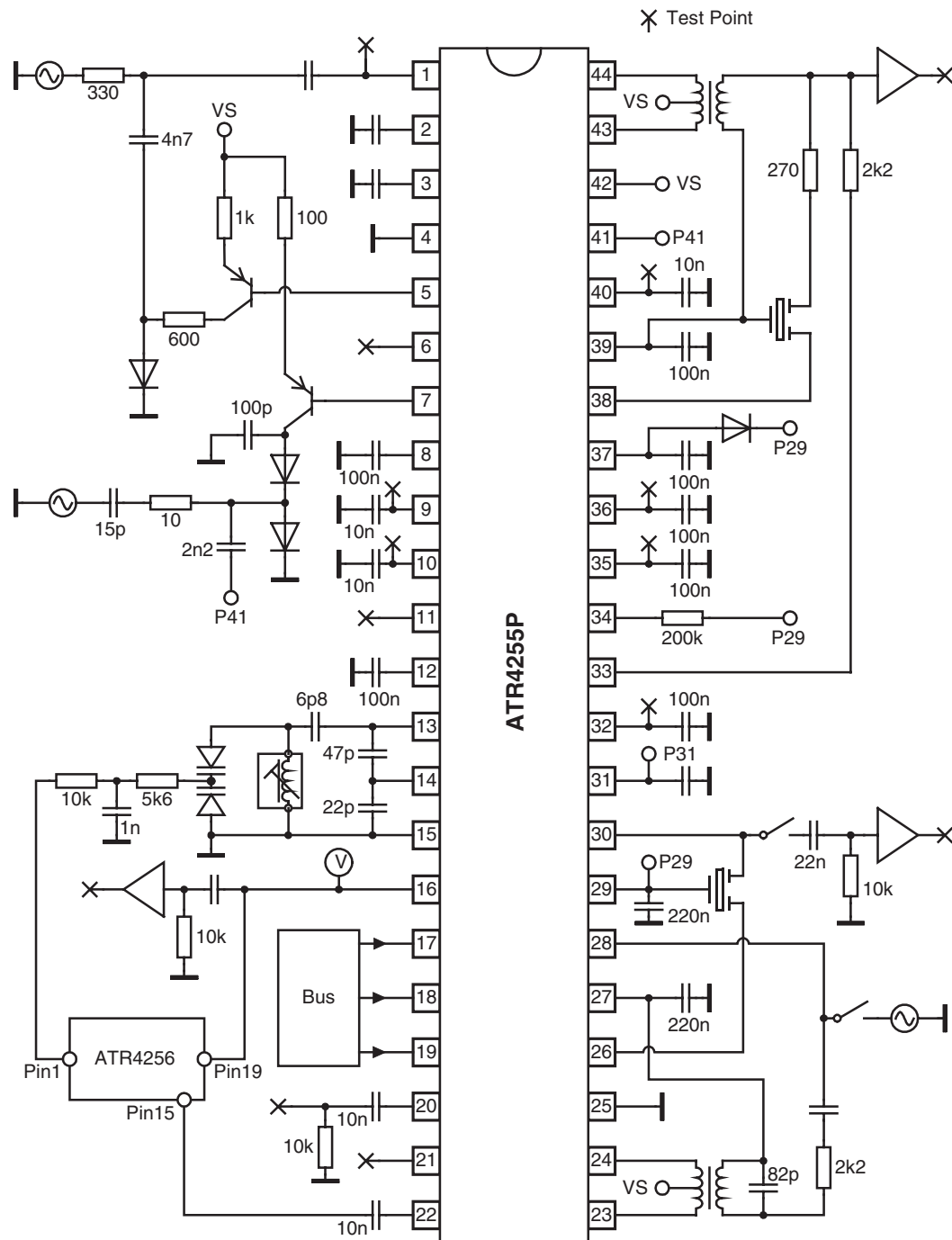
Figure 8-8. Test Circuit
