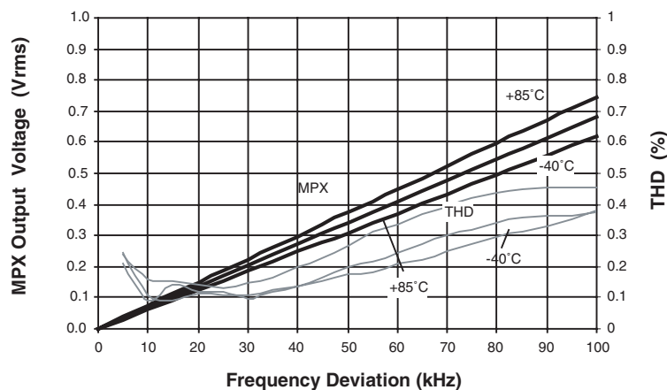
Figure 8-1. FM Demodulator
