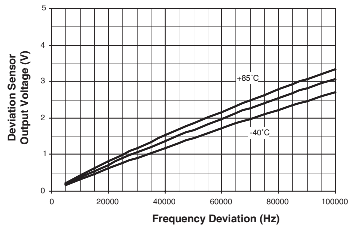
Figure 8-4. Deviation Sensor
