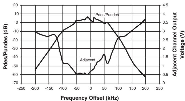
Figure 8-7. Selectivity
