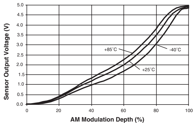
Figure 8-2. Multipath Sensor
