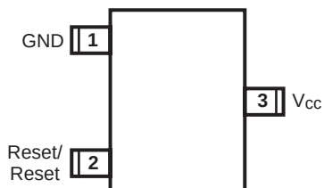
Pin Configuration SOT-23 (Top View)
