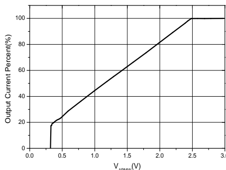
Figure 3: Analog Dimming Curve
