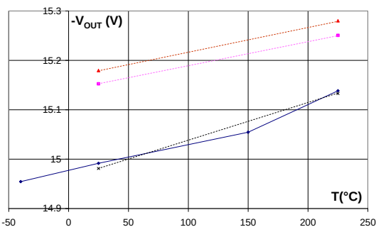
Figure 4: -V_{out} vs. T^\circ (dropout=2V ; I_{load}=60mA , 4 samples)
