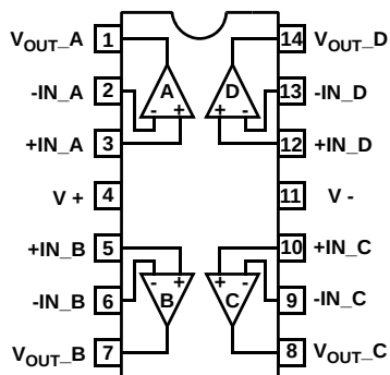
ISL28407 (14 LD SOIC) TOP VIEW
