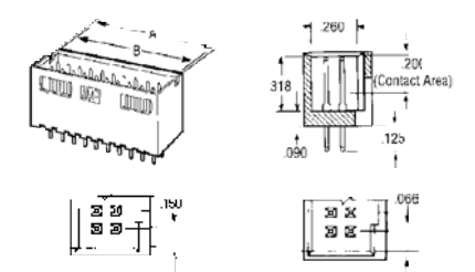
.025 Square Straight Post — .066 End Dimension †100-499
