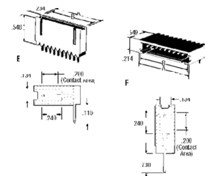
.025 Sq. Straight Post (with Standoffs) — Fig. E †100-499
