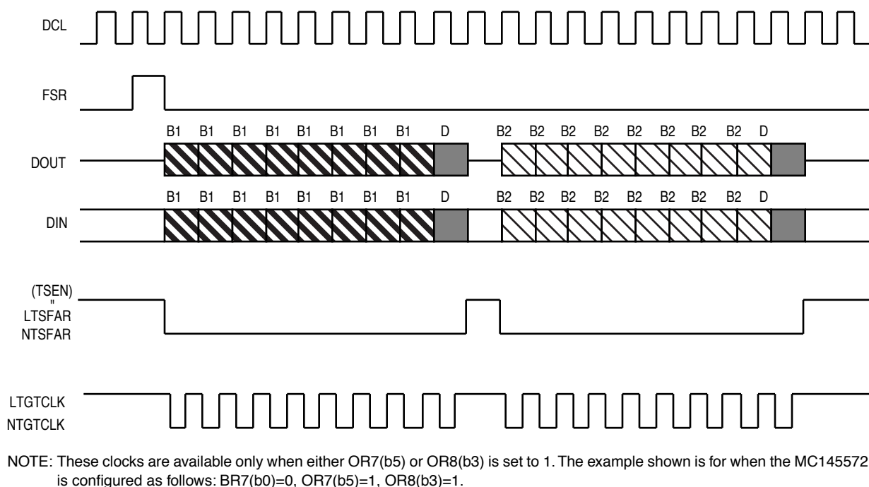
Figure 2-6. BERT Gated Clock — 10-Bit Gated Clock
