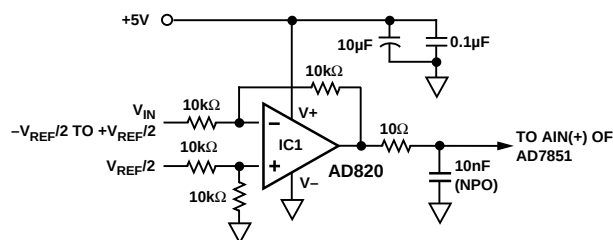
Figure 13. Analog Input Buffering
