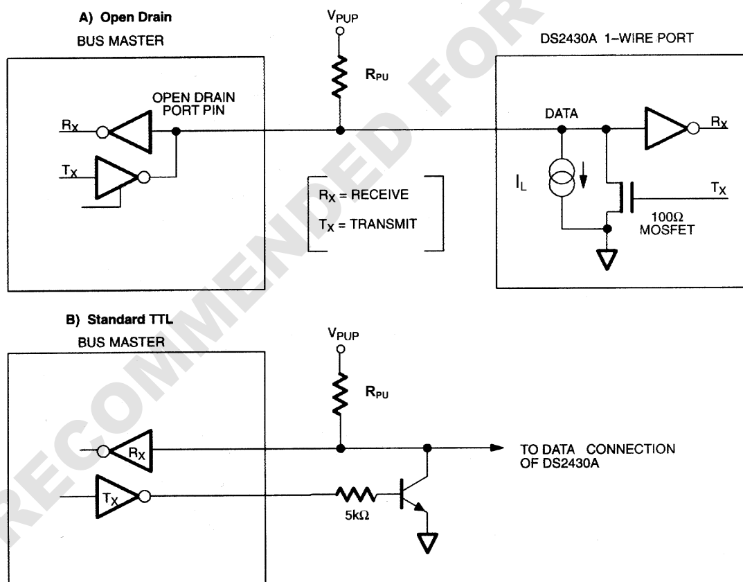
HARDWARE CONFIGURATION Figure 7
