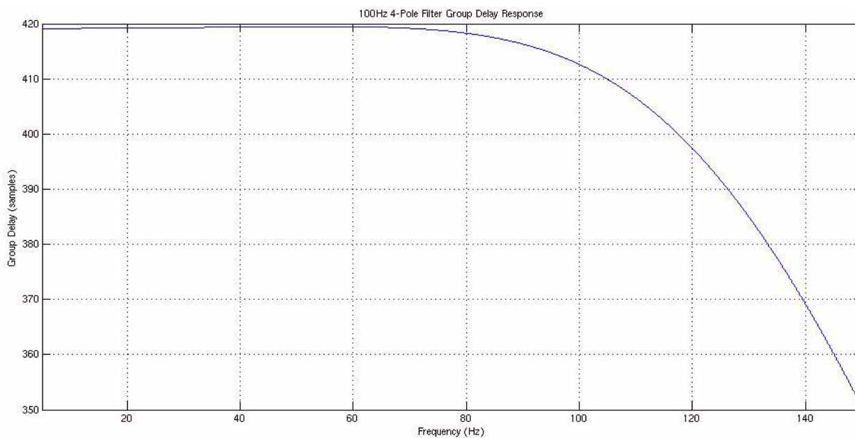
Figure 14. Low-Pass Filter Characteristics: f_C = 100 Hz, Poles = 4, t_S = 8 \mu s
