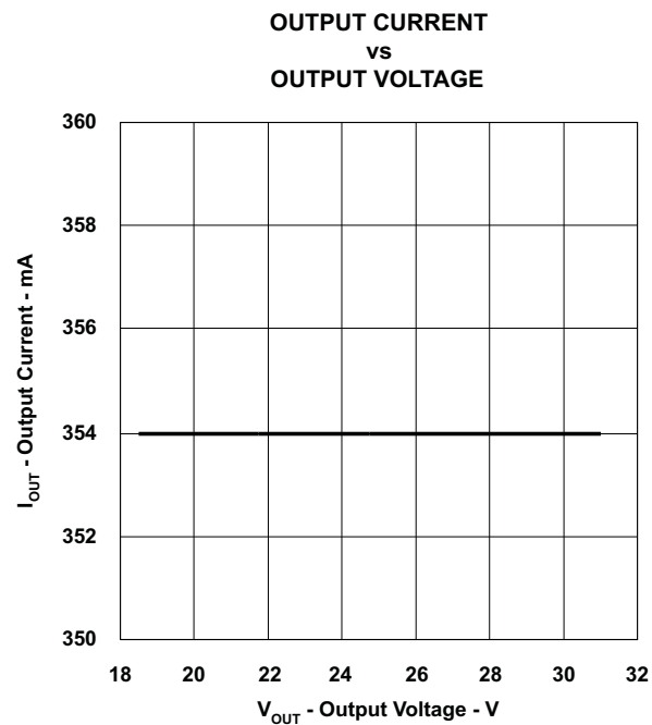
Figure 7. Load Regulation
