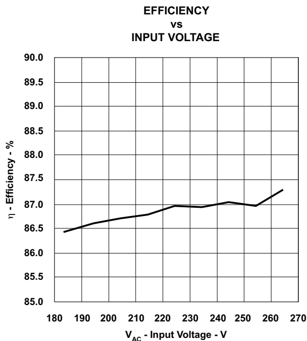
Figure 4. Efficiency
