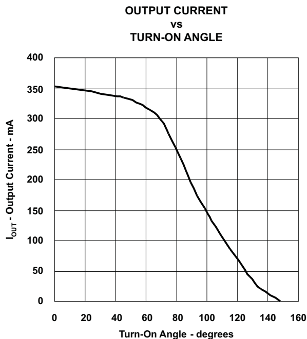
Figure 9. TRIAC Dimmer Performance
