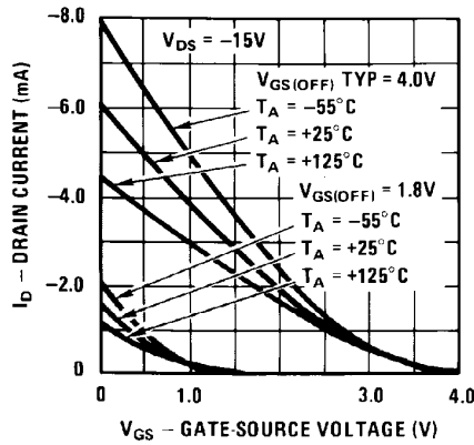
Figure 1. Transfer Characteristics
