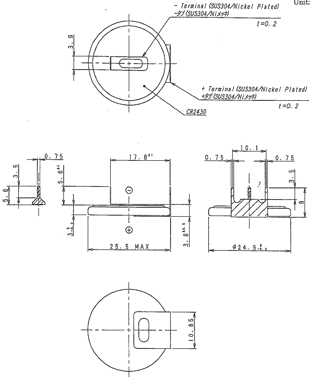
Fig.1 Shape and Dimensions Item : CR2430-F2AW3
