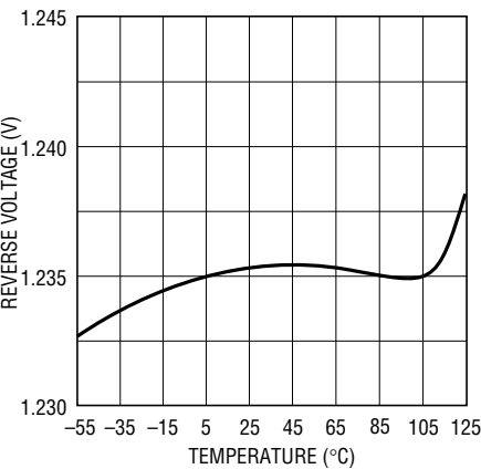
Temperature Drift
