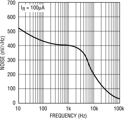
Noise Voltage
