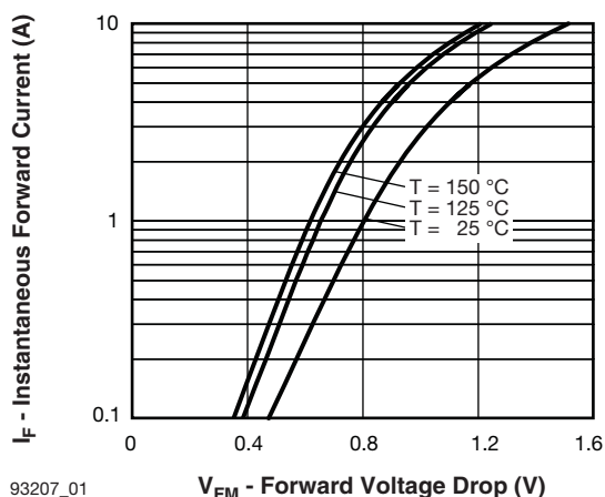
93207_01 Fig. 1 - Maximum Forward Voltage Drop Characteristics
