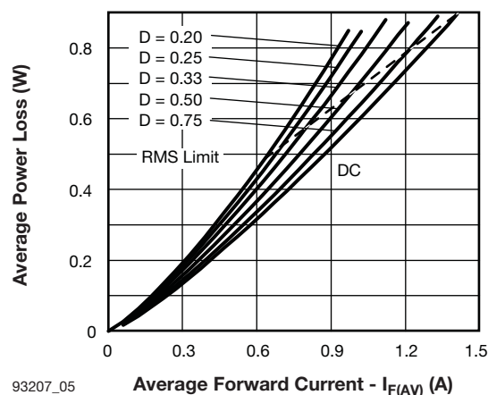
93207_05 Fig. 5 - Forward Power Loss Characteristics
