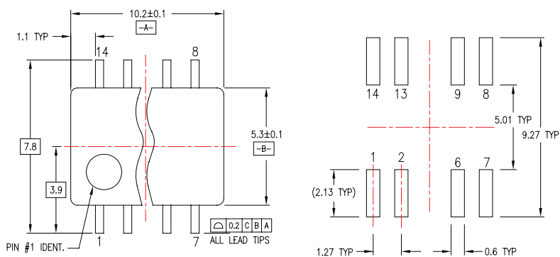
LAND PATTERN RECOMMENDATION
