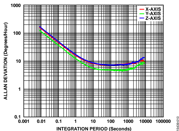
Figure 10. Gyroscope Allan Deviation, T_C = 25^\circ\text{C} , ADIS16467-3
