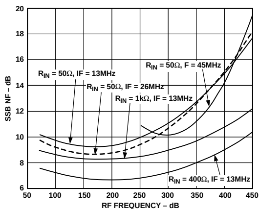
Figure 3. Mixer Noise Figure vs. RF Frequency
