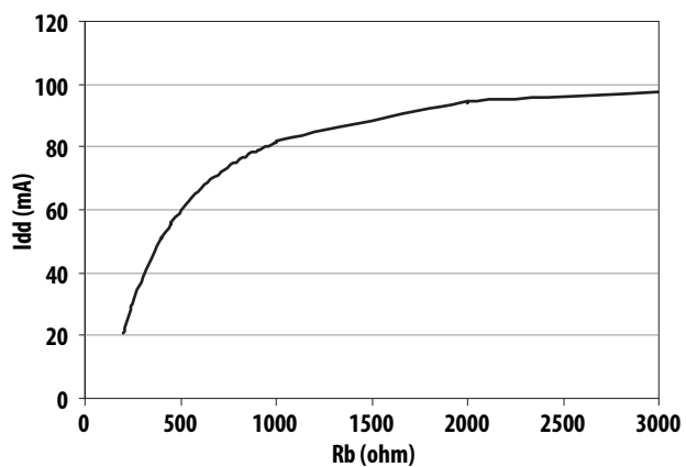
Figure 23. Idd vs Rb
