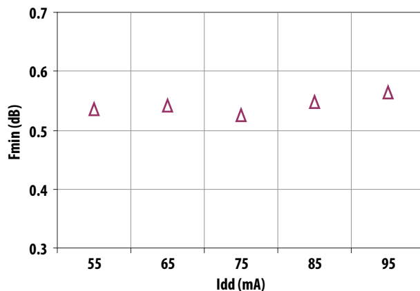
Figure 8. F_{min} vs I_{DD} at 4.8 V at 1.9 GHz
