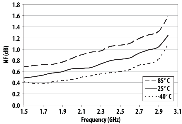
Figure 17. NF vs Frequency vs Temperature
