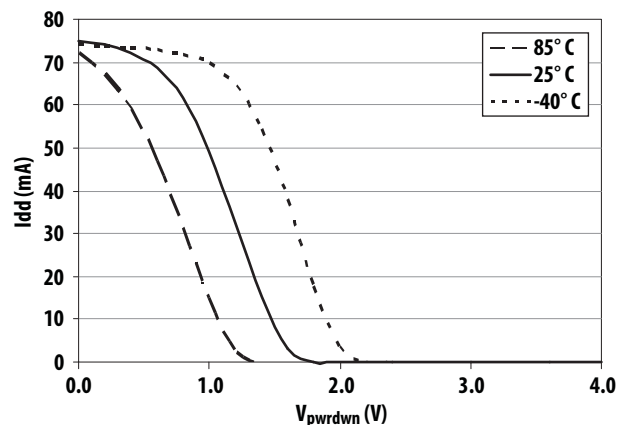
Figure 24. Idd vs V_{pwrdown}
