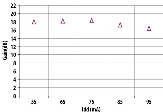
Figure 9. Gain vs I_{DD} at 4.8 V Tuned for Optimum IIP3 and F_{min} at 1.7 GHz
