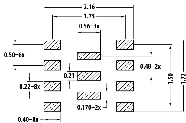
Stencil Design
