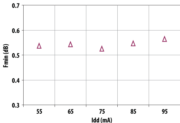
Figure 7. F_{min} vs I_{DD} at 4.8 V at 1.7 GHz
