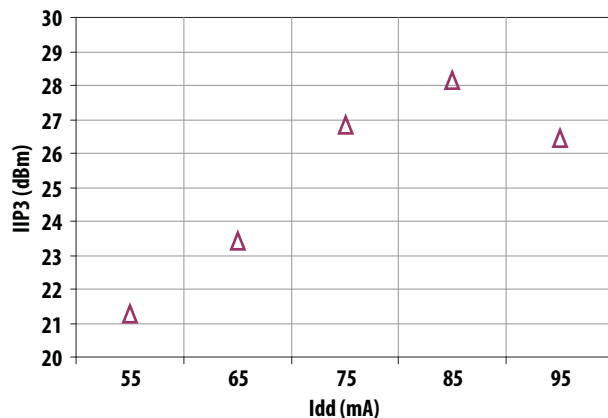
Figure 12. IIP3 vs I_{DD} at 4.8 V Tuned for Optimum IIP3 and F_{min} at 1.9 GHz
