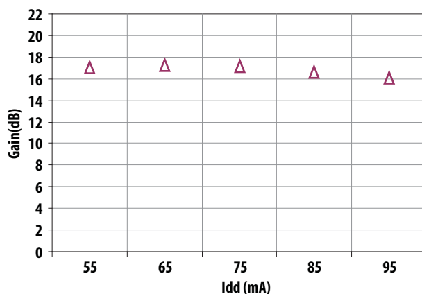
Figure 10. Gain vs I_{DD} at 4.8 V Tuned for Optimum IIP3 and F_{min} at 1.9 GHz
