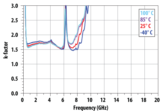
Figure 22. k-factor vs Frequency vs Temperature
