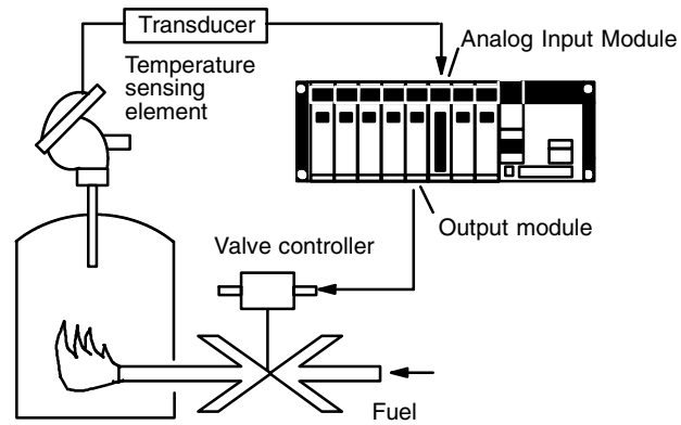
Furnace Control with Analog Input
