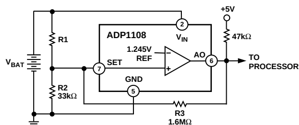
Figure 24b. Adding Hysteresis to the Low Battery Detector
