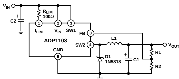
Figure 16. Step-Down Mode Operation
