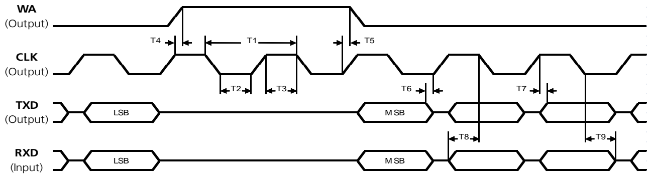
Figure 9: AC characteristics of digital audio interface in PCM mode (<l2s_mode> = 0) and Master mode enabled
