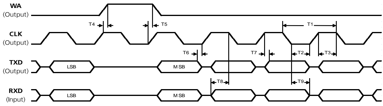
Figure 10: AC characteristics of digital audio interface in PCM mode (<l2s_mode> = 1) and Master mode enabled
