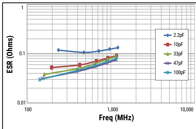
ESR vs. Frequency 0805
