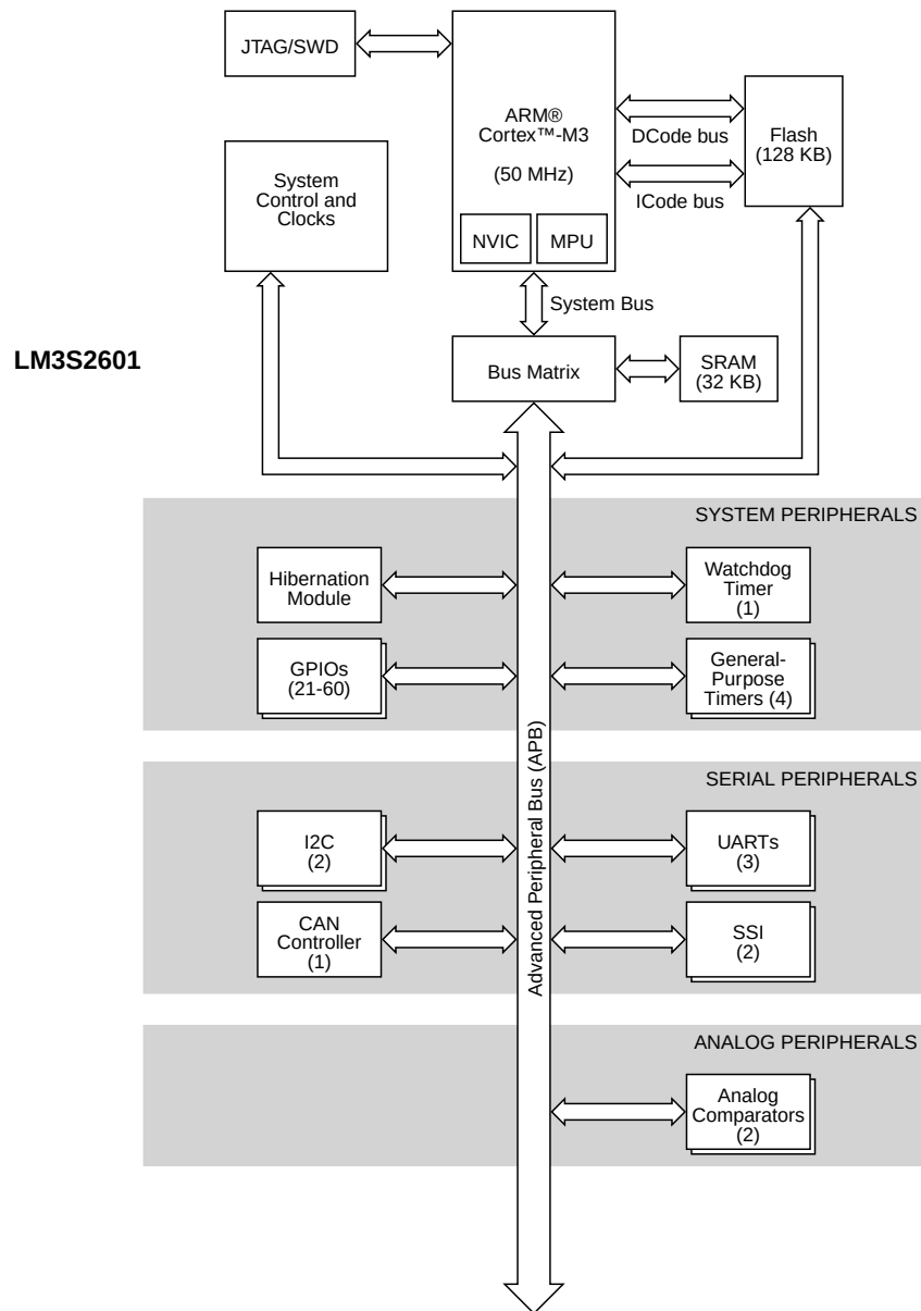
Figure 1-1. Stellaris® LM3S2601 Microcontroller High-Level Block Diagram
