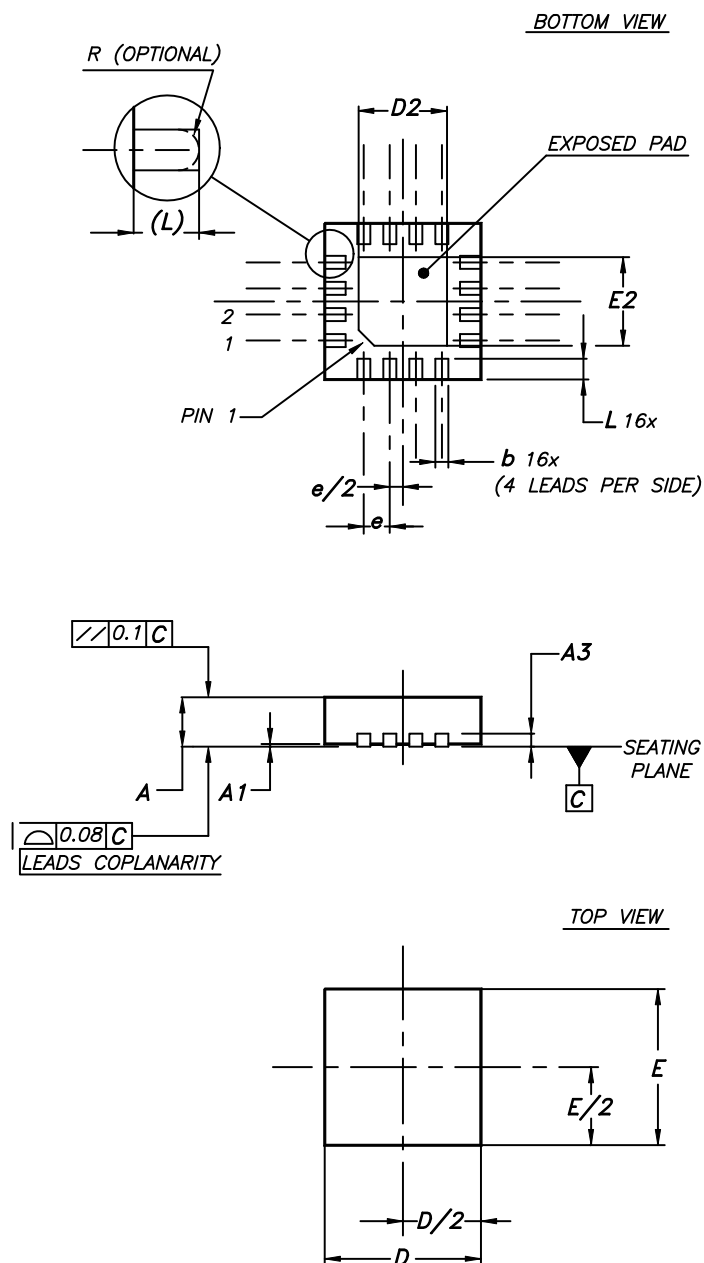
Figure 46. QFN16 3x3 package outline
