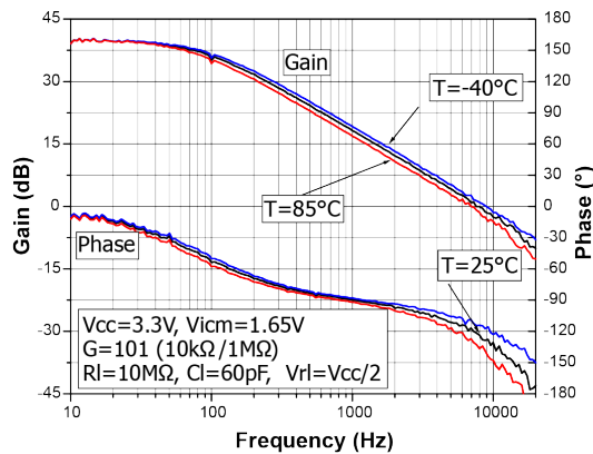
Figure 28. Bode diagram at 3.3 V supply voltage
