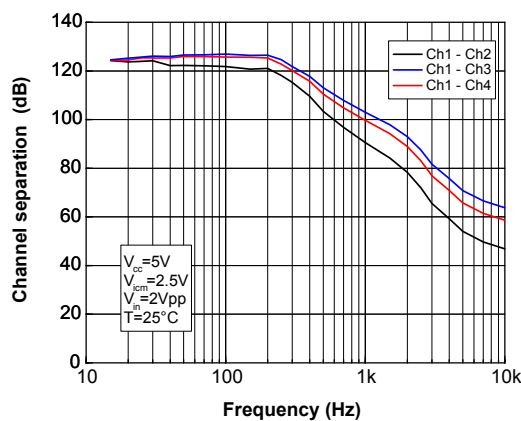
Figure 37. Channel separation on TSU104
