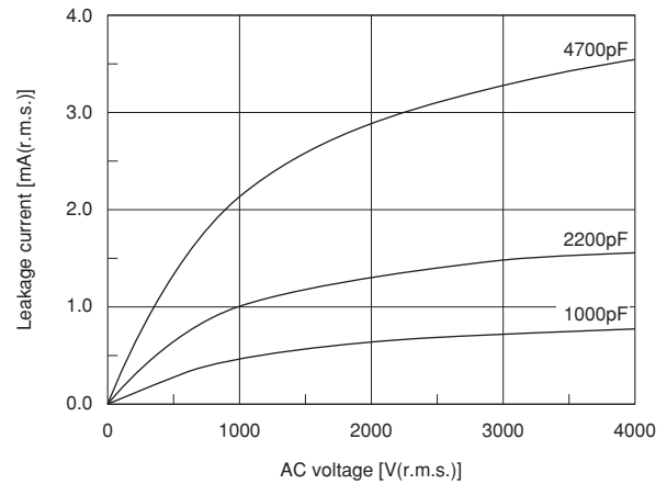
Type KJ (E char.)
