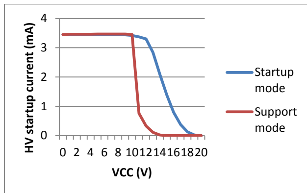
Figure 1: HV regulator characteristics
