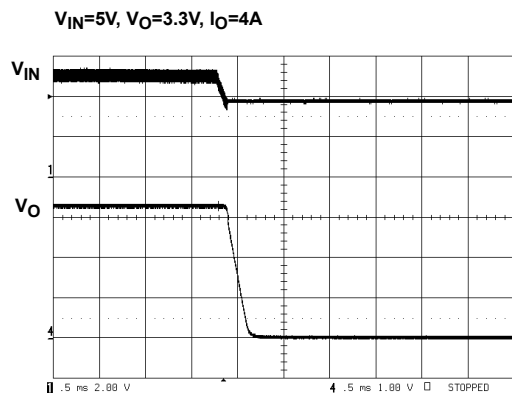
FIGURE 17. POWER-DOWN
