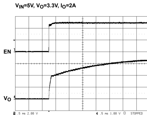
FIGURE 18. RELEASING EN
