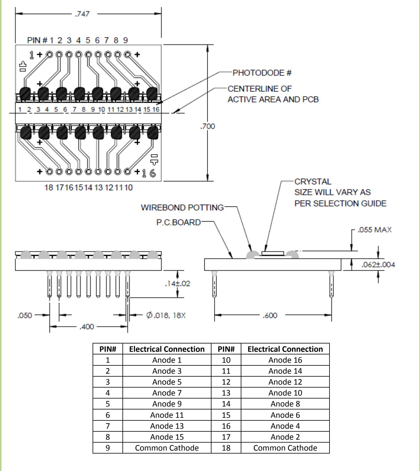
VTA1216H-L (Dimensions are in inches)
