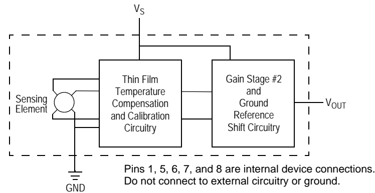
Figure 1. Integrated pressure sensor schematic
