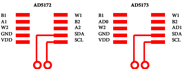
Figure 38. Recommended AD5172/73 PCB Layout. The SCL and SDA pads allow pogo pins to be inserted so that signals can be communicated through the parallel port for programming (Figure 37).
