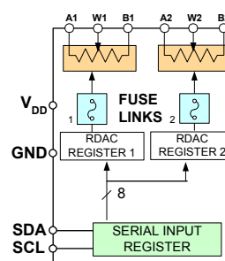
Figure 1. AD5172
