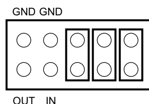
Figure 2. CN002 Pinout
