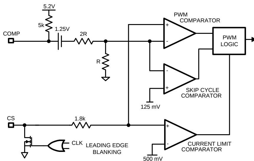
Figure 13. Skip Cycle Control
