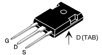
TO-247 AD
