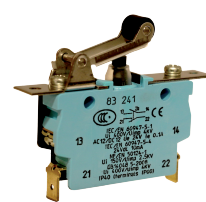
Mixed connections: NO screw with clamp / NC quick-connect 6.3 x 0.8, 90° downward folding
