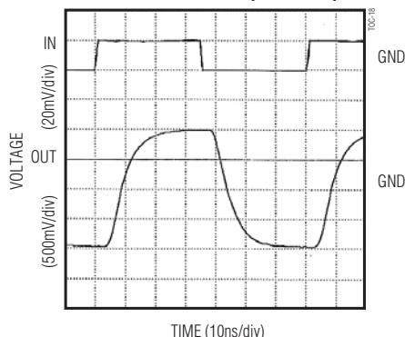
MAX4146 LARGE-SIGNAL PULSE RESPONSE ( A_V = +100 )
