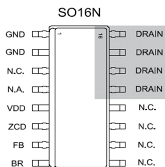
Figure 3. Pin description
