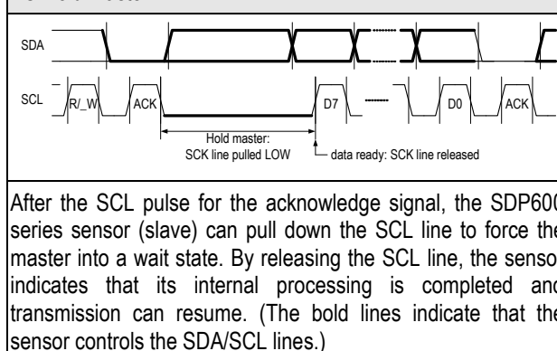
I 2 C Hold Master
