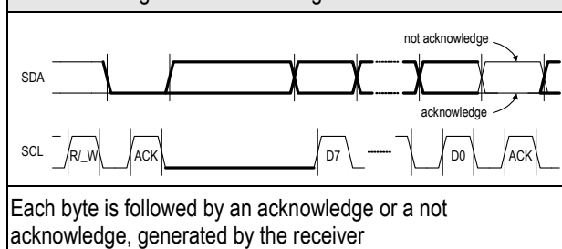
I 2 C Acknowledge / Not Acknowledge
