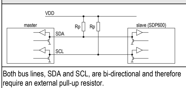
I 2 C Transmission Start Condition
