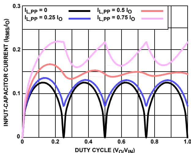
FIGURE 19. NORMALIZED INPUT-CAPACITOR RMS CURRENT vs DUTY CYCLE FOR 4-PHASE CONVERTER
