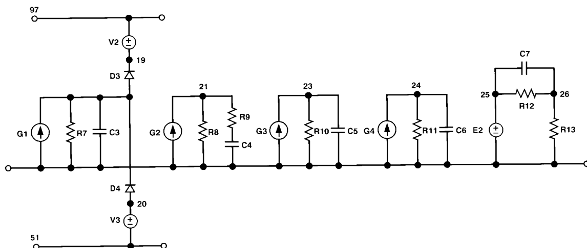
Spice Diagram (B)
