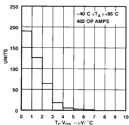
t_C V_{OS} Distribution
