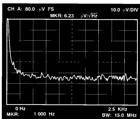
OP-285 Voltage Noise Density vs. Frequency V_S = \pm 15\text{ V} , A_V = 1000
