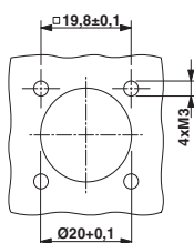
Einbaumaße: RF-1.S..8AAAF00 , RF-1.P..8AAAF00
