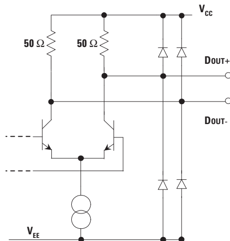
Figure 12. Receiver data output equivalent circuit
