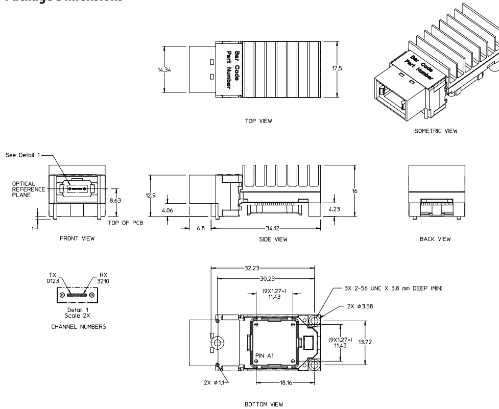
Figure 4A. HFBR-7924 Package dimensions (dimensions in mm)
