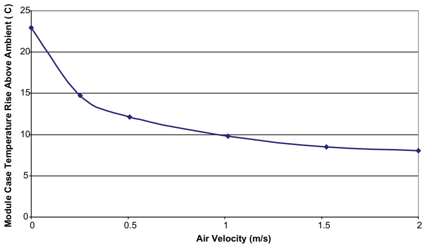
Figure 3. Ambient air temperature and air flow for T_C = +80^\circ\text{C}
