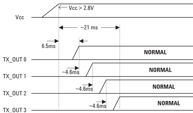
Figure 17. Typical Transmitter Power-Up Sequence
