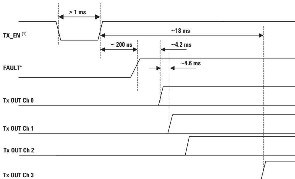
Figure 15. Transmitter TX_EN and TX_DIS timing diagram
