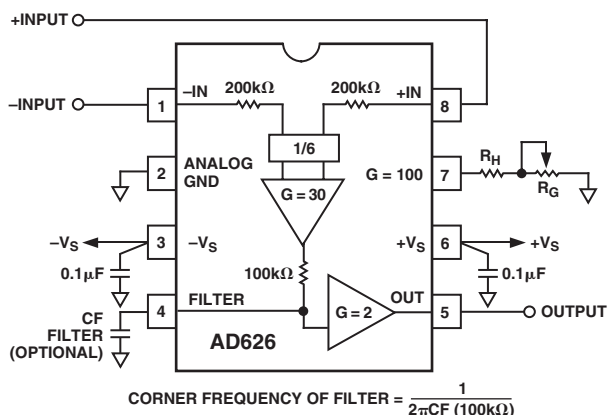
RESISTOR VALUES FOR GAIN ADJUSTMENT
