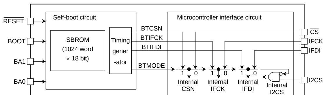
Figure 1 Self-Boot System
