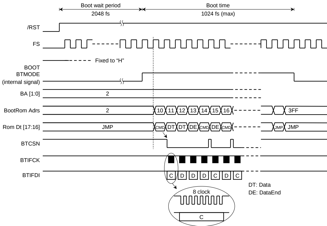
Figure 3 Boot Timing Chart (at reset)
