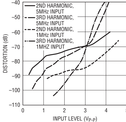
Distortion vs Signal Level V_S = \pm 5V , R_L = 800\Omega at Each Output, T_A = 25^\circ C
