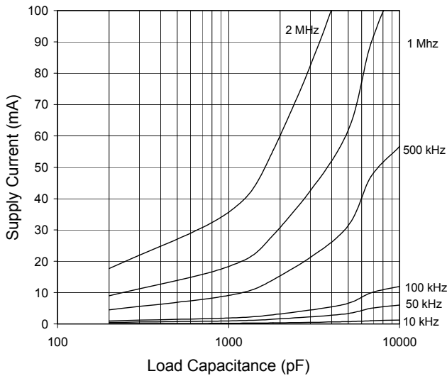
Fig. 15 Supply Current vs. Load Capacitance Vcc = 18V
