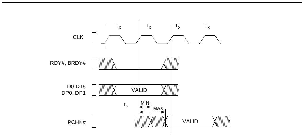
Figure 13. PCHK# Valid Delay Timing
