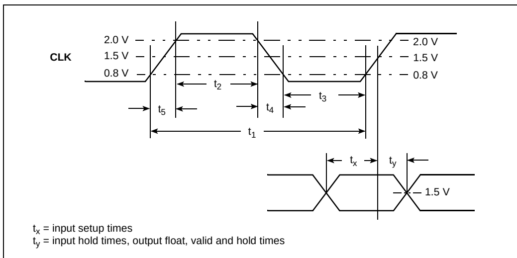
Figure 9. CLK Waveform
