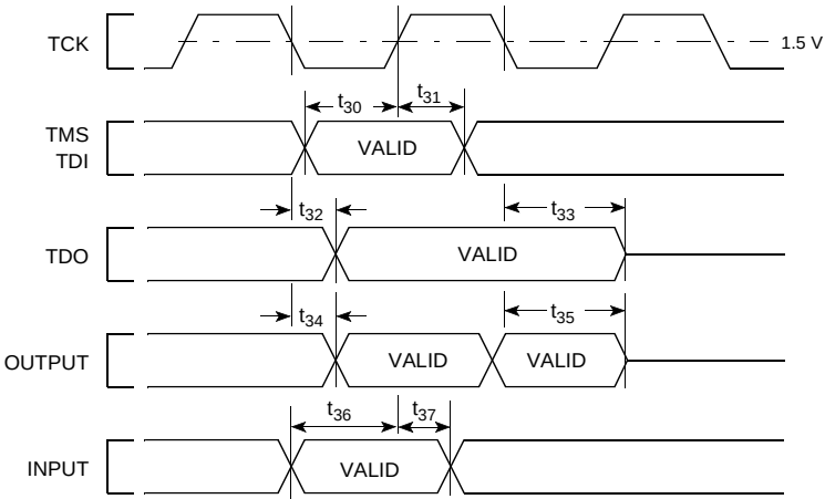
Figure 16. Test Signal Timing Diagram
