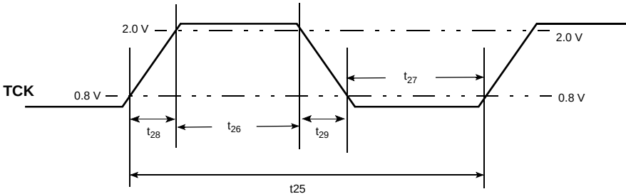
Figure 15. TCK Waveform
